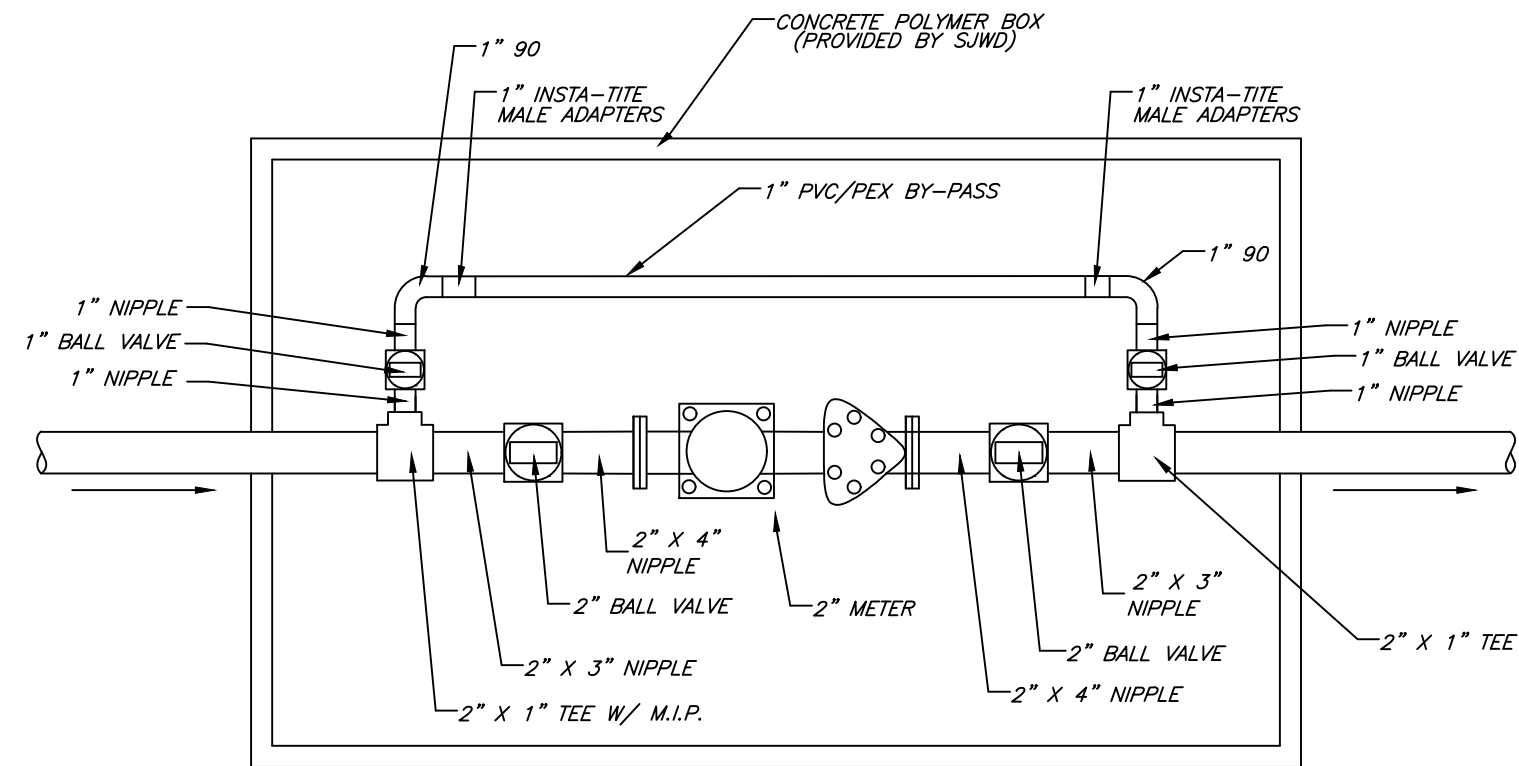
2" METER PLAN
