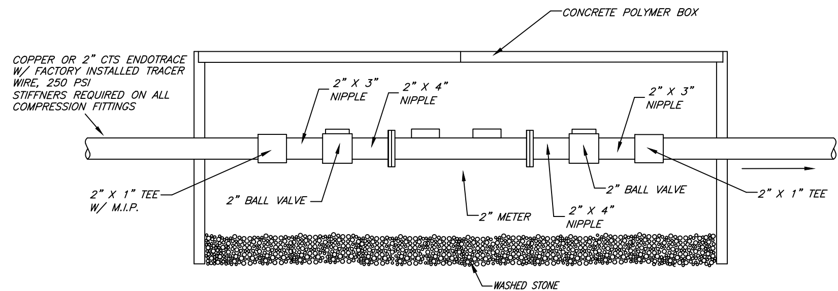
2" METER PROFILE
